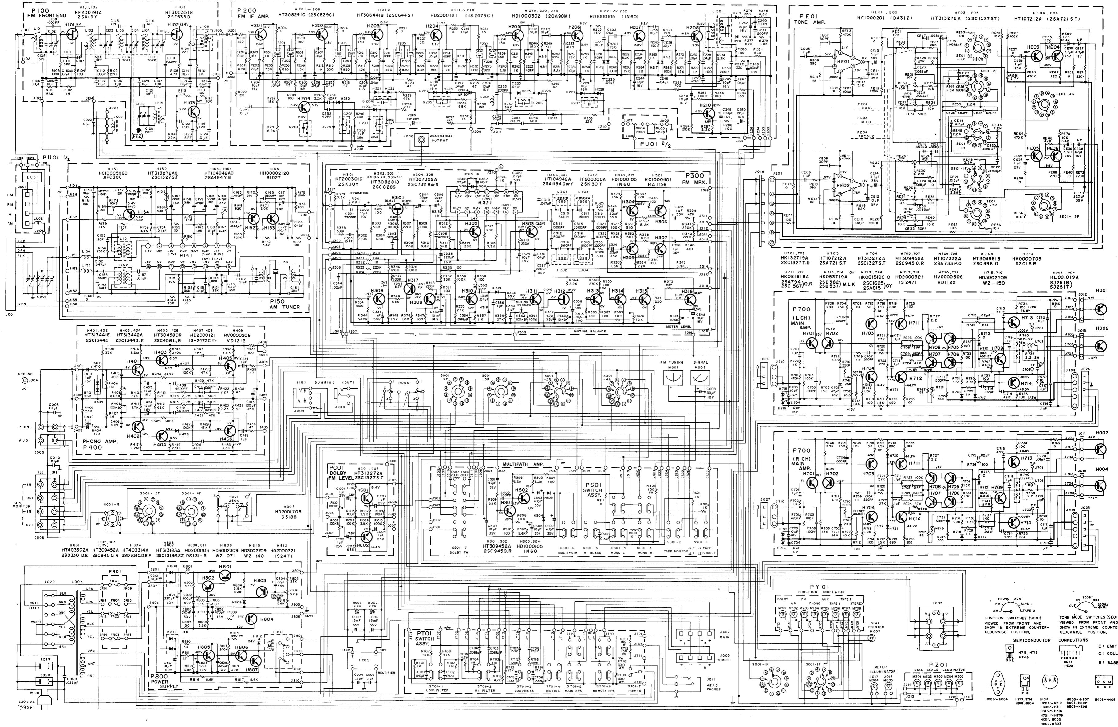
Figure 27. Schematic Diagram for European Model
